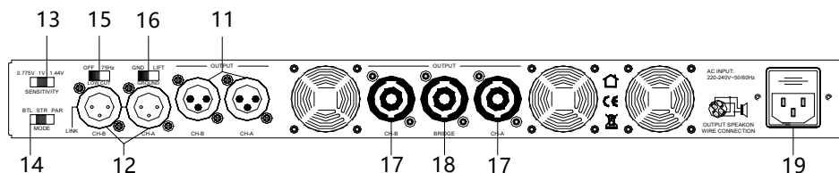
PV2030 Rear Panel
